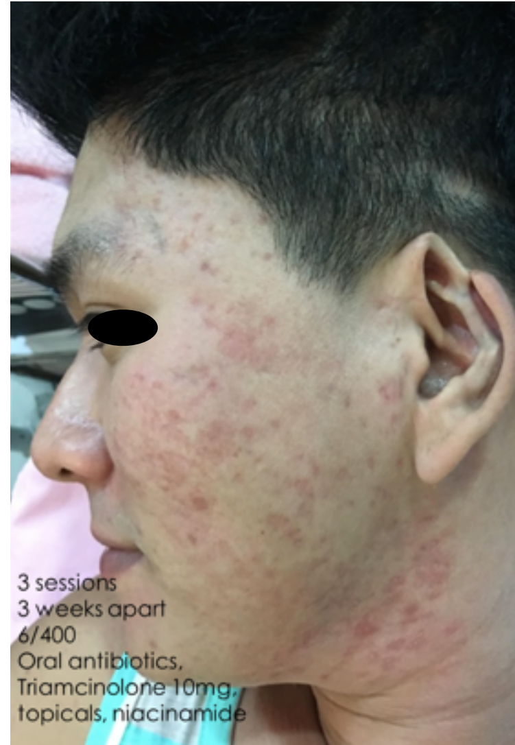
3 Tixel treatments
